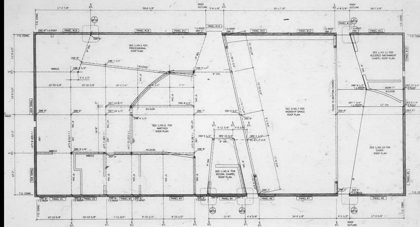
planta / floor plan
