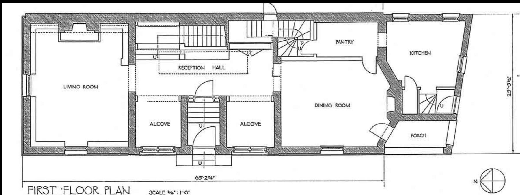
Charnley House— Chicago — 1891-1892
