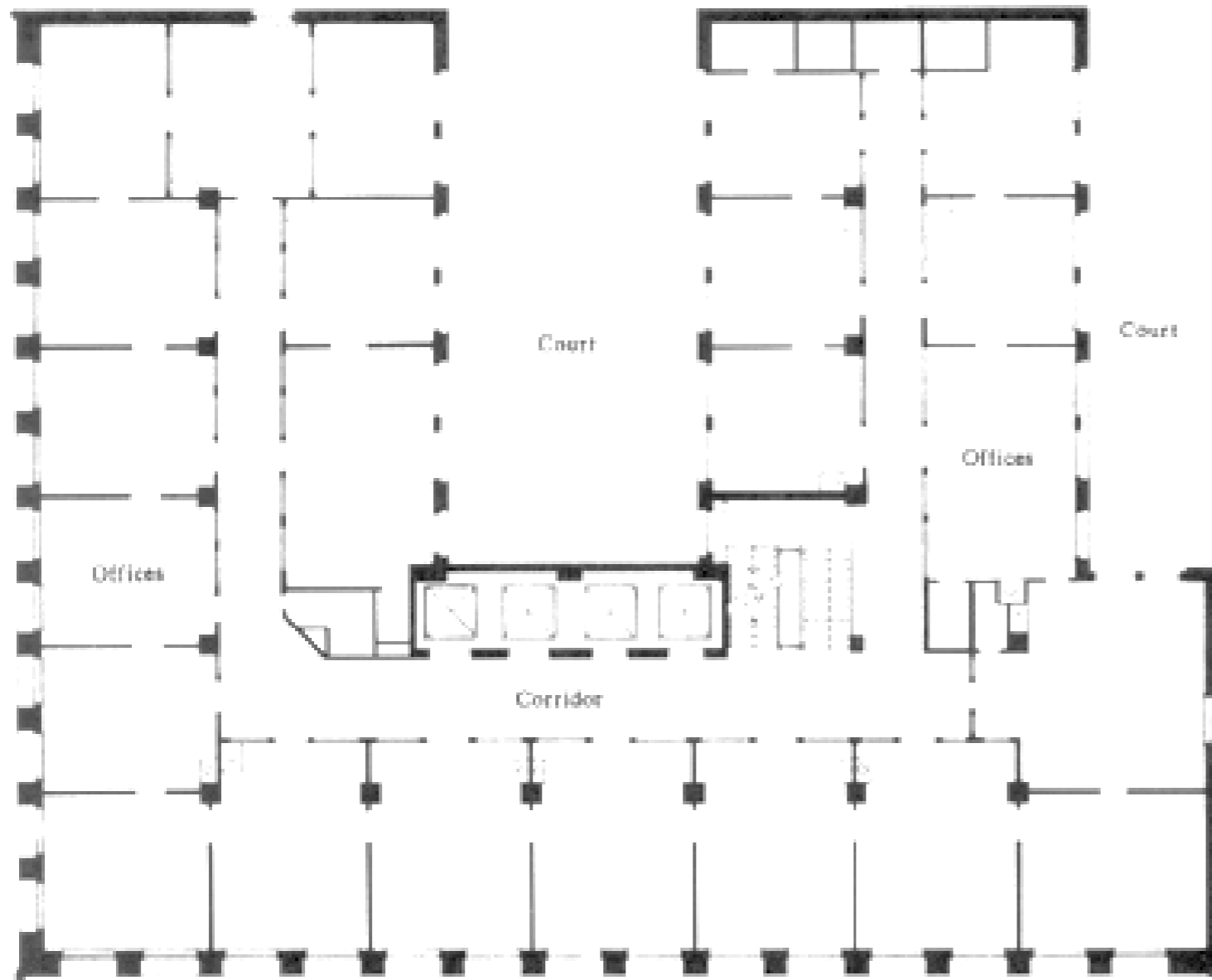
TYPICAL UPPER FLOOR PLAN, 1897
