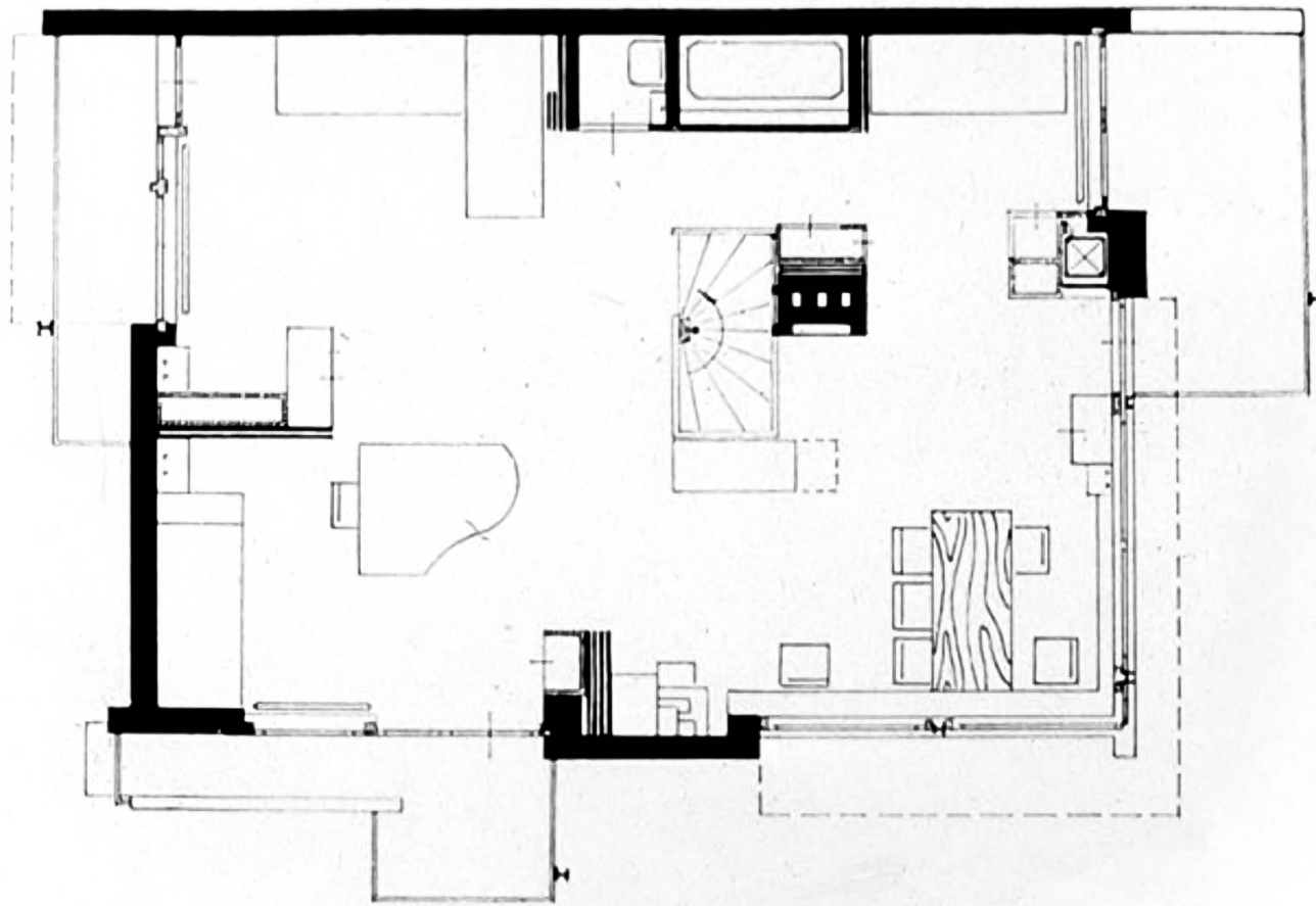
Schröder house plan, first floor (open)
