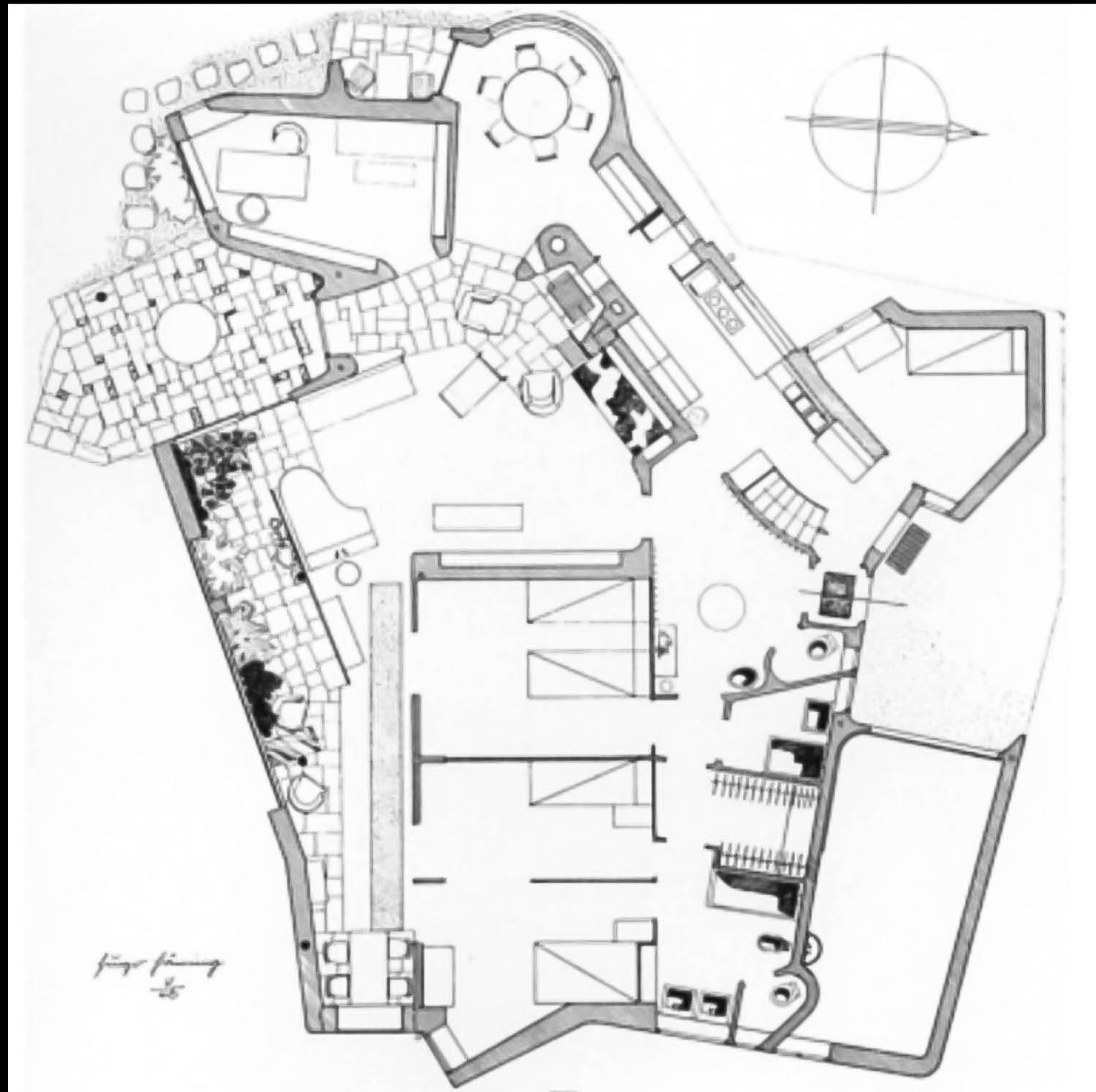
Theoretical House Plan | Hugo Häring | 1946
